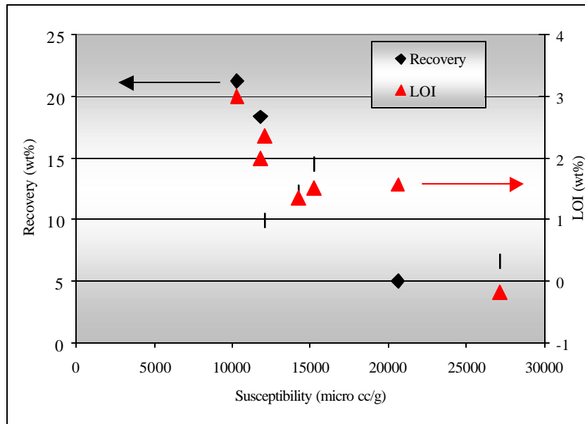
Figure 1. Recovery and LOI for Fly Ash B 2 as a Function of Magnetic Susceptibility
